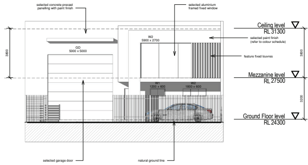
① East Elevation 1 : 100
